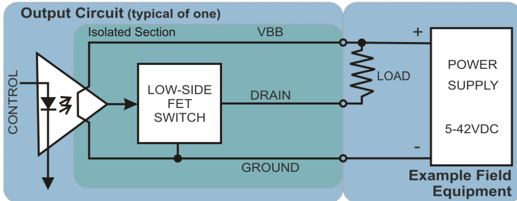
Figure 1-3: Example of One Output Circuit
